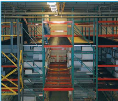
Rack-Supported Catwalk Mezzanine (Two-Level)
